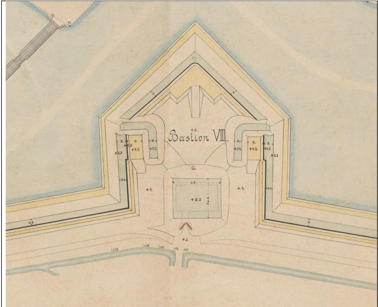
Plattegrond Bastion VIII
